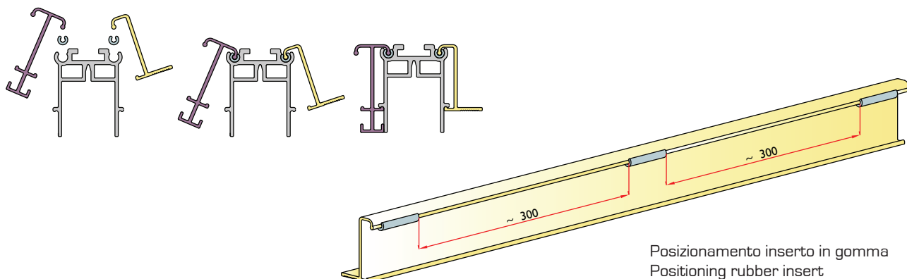
Sistema per aggancio profili in alluminio System for connection aluminium profiles
