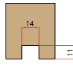
Binario in plastica Plastic Track Art.760/N
